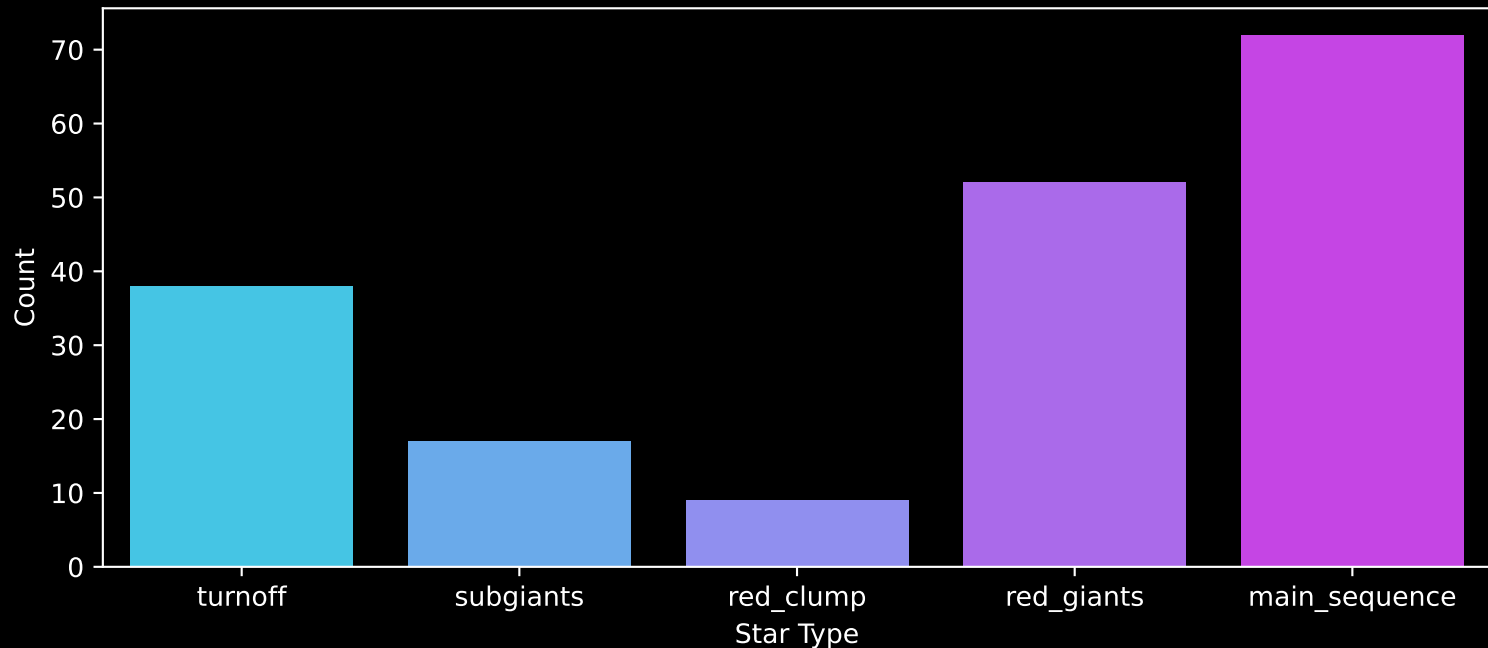
APOGEE DR17 Field: [176+27_MGA] Count plot of Star Type
