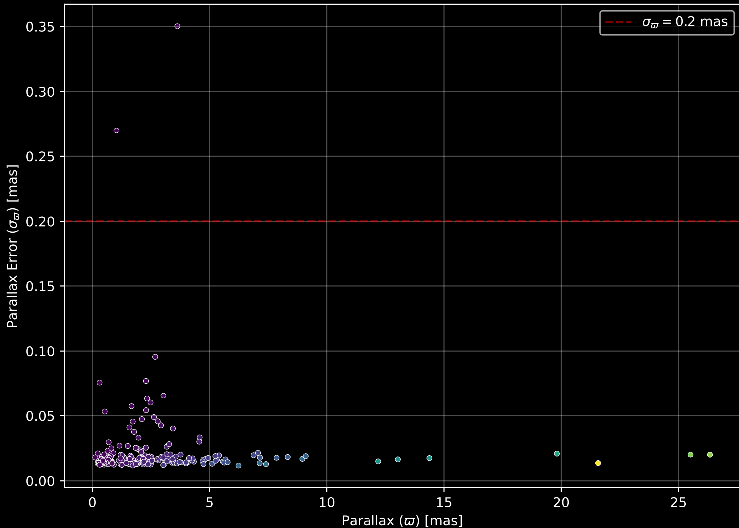
APOGEE DR17 Field: [176+27_MGA] Parallax Quality (n= 188)
