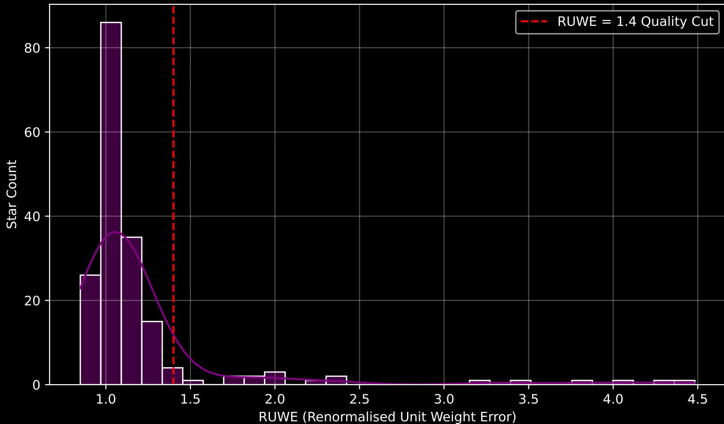
GAPOGEE DR17 Field [176+27_MGA] RUWE Distribution (n= 183)
