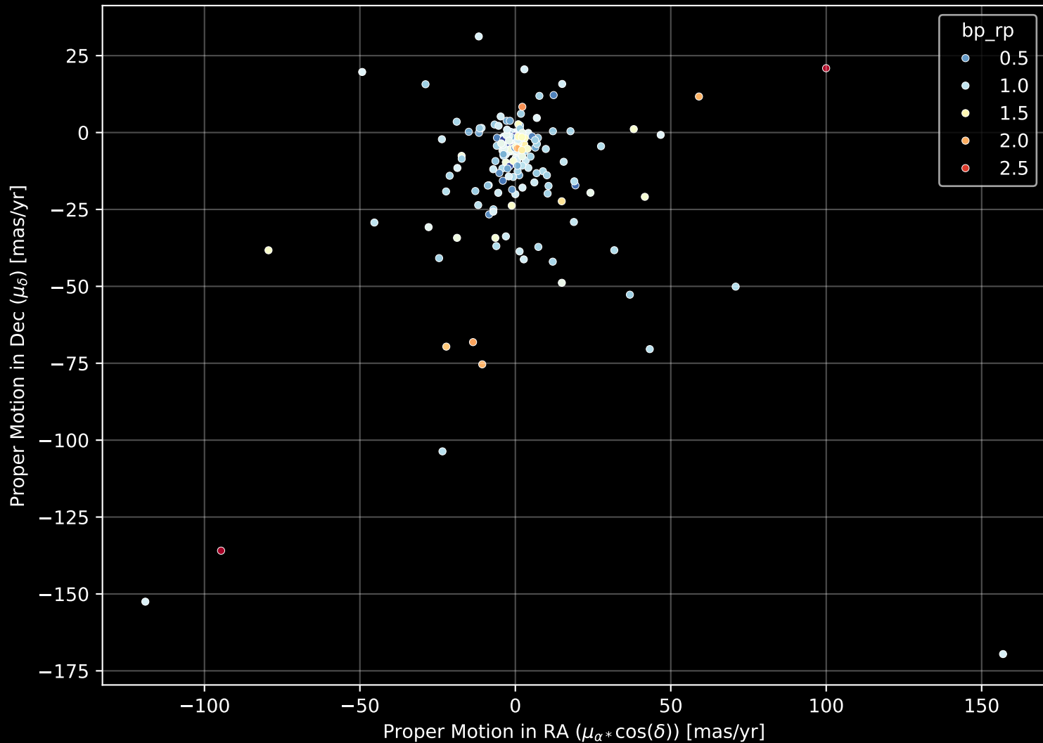
APOGEE DR17 Field: [176+27_MGA] Proper Motion Diagram (n= 188)
