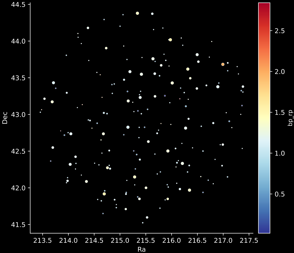
APOGEE DR17 Field: [176+27_MGA] Stars: 188
