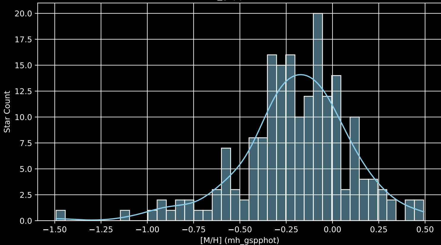
APOGEE DR17 Field: [176+27_MGA [M/H] (mh_gspphot) (n= 188)
