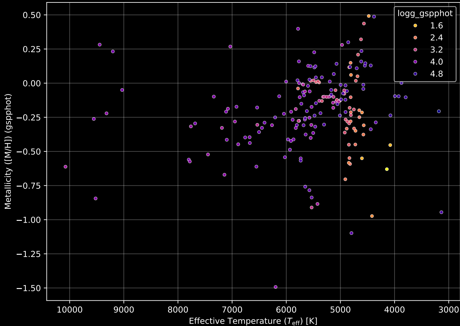
APOGEE DR17 Field: [176+27_MGA] Stellar Population Parameters (n= 188)
